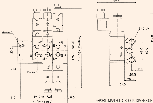
5-PORT MANIFOLD BLOCK DIMENSION n = STATION
